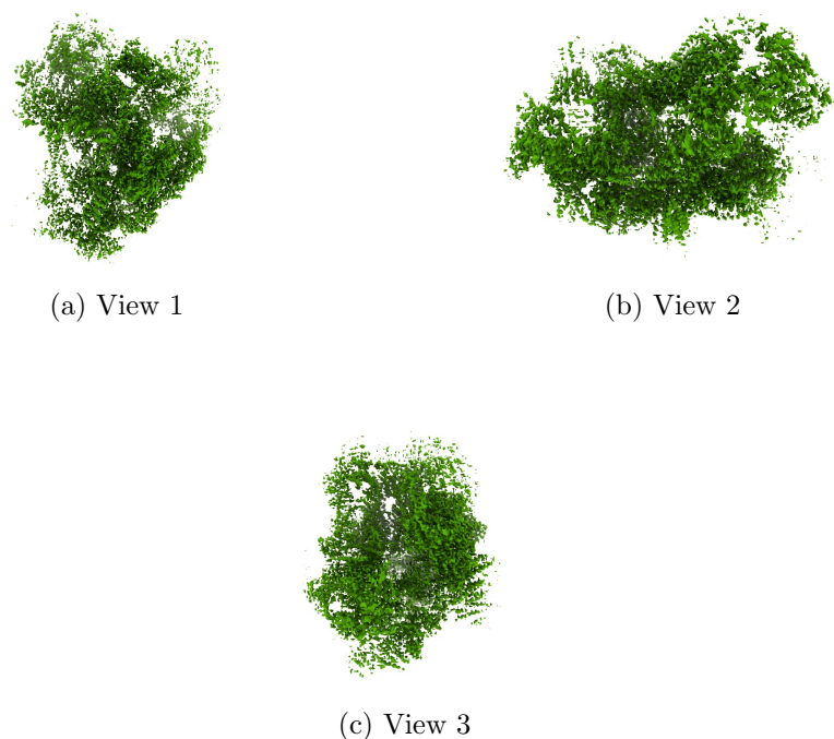
Figure 4: Isosurface at threshold=0.754000. Views generated by ChimeraX at a the following X, Y, Z angles: View 1 (0, -90, -90), View 2 (-90, 0, -90), View 3 (0, 0, 0).
