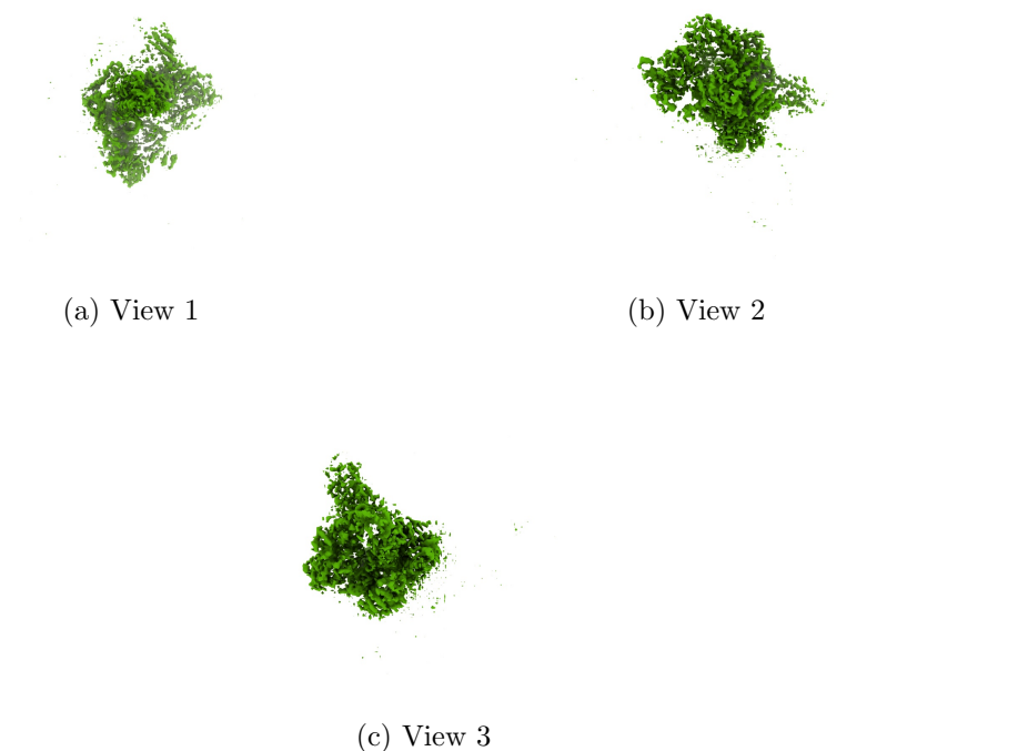
Figure 4: Isosurface at threshold=0.519600. Views generated by ChimeraX at a the following X, Y, Z angles: View 1 (0, -90, -90), View 2 (-90, 0, -90), View 3 (0, 0, 0).
