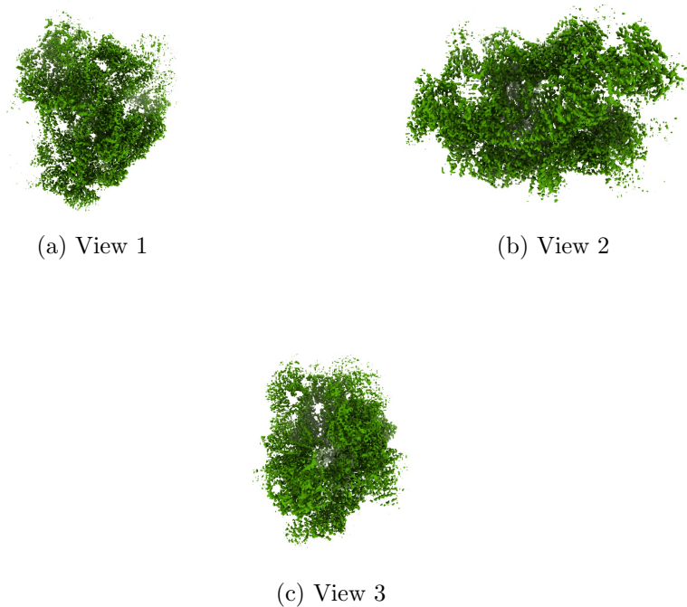
Figure 4: Isosurface at threshold=0.753600. Views generated by ChimeraX at a the following X, Y, Z angles: View 1 (0, -90, -90), View 2 (-90, 0, -90), View 3 (0, 0, 0).
