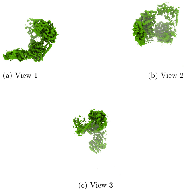
Figure 4: Isosurface at threshold=0.480800. Views generated by ChimeraX at a the following X, Y, Z angles: View 1 (0, -90, -90), View 2 (-90, 0, -90), View 3 (0, 0, 0).
