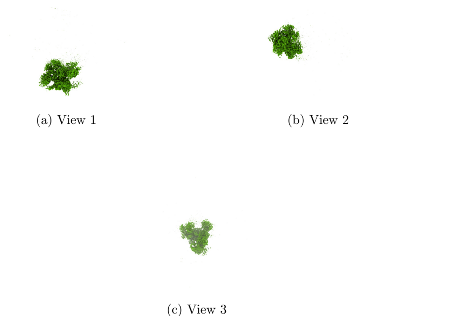
Figure 4: Isosurface at threshold=0.594000. Views generated by ChimeraX at a the following X, Y, Z angles: View 1 (0, -90, -90), View 2 (-90, 0, -90), View 3 (0, 0, 0).
