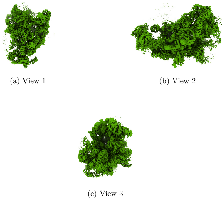
Figure 4: Isosurface at threshold=0.293500. Views generated by ChimeraX at a the following X, Y, Z angles: View 1 (0, -90, -90), View 2 (-90, 0, -90), View 3 (0, 0, 0).
