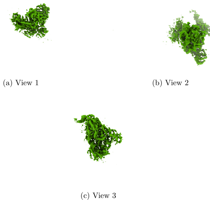
Figure 4: Isosurface at threshold=0.479000. Views generated by ChimeraX at a the following X, Y, Z angles: View 1 (0, -90, -90), View 2 (-90, 0, -90), View 3 (0, 0, 0).
