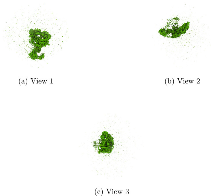
Figure 4: Isosurface at threshold=0.246100. Views generated by ChimeraX at a the following X, Y, Z angles: View 1 (0, -90, -90), View 2 (-90, 0, -90), View 3 (0, 0, 0).
