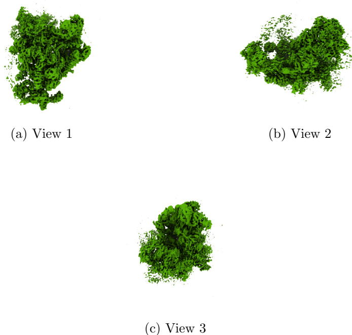
Figure 4: Isosurface at threshold=0.273600. Views generated by ChimeraX at a the following X, Y, Z angles: View 1 (0, -90, -90), View 2 (-90, 0, -90), View 3 (0, 0, 0).
