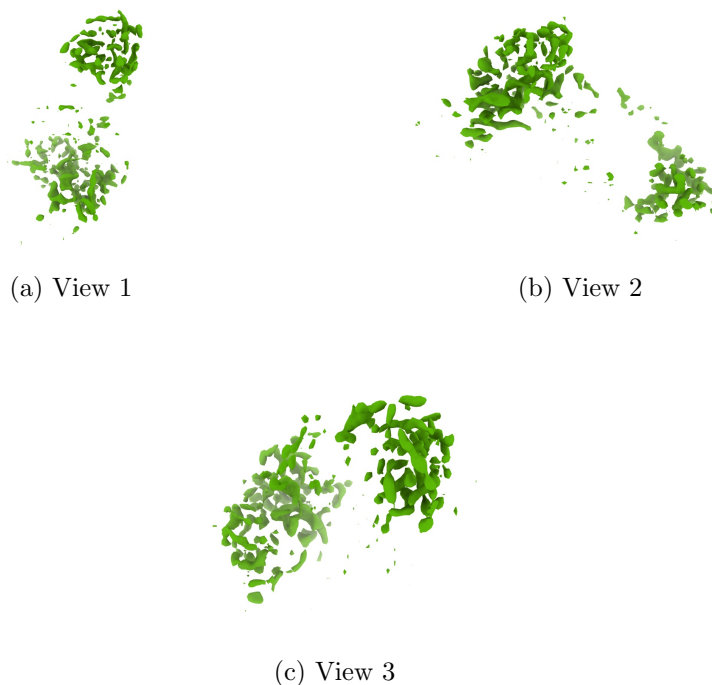
Figure 4: Isosurface at threshold=0.948000. Views generated by ChimeraX at a the following X, Y, Z angles: View 1 (0, -90, -90), View 2 (-90, 0, -90), View 3 (0, 0, 0).
