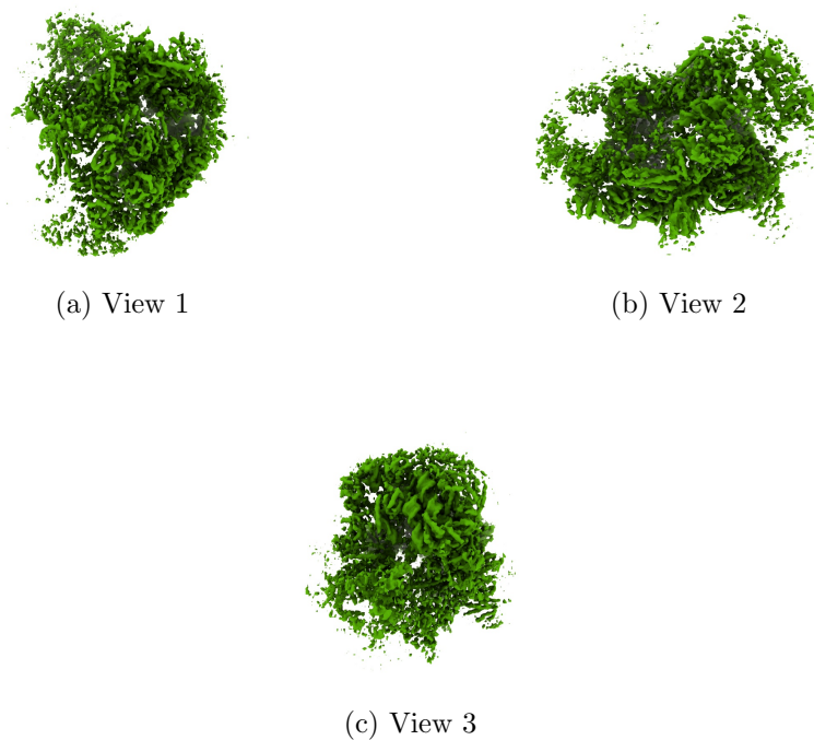
Figure 4: Isosurface at threshold=0.448800. Views generated by ChimeraX at a the following X, Y, Z angles: View 1 (0, -90, -90), View 2 (-90, 0, -90), View 3 (0, 0, 0).
