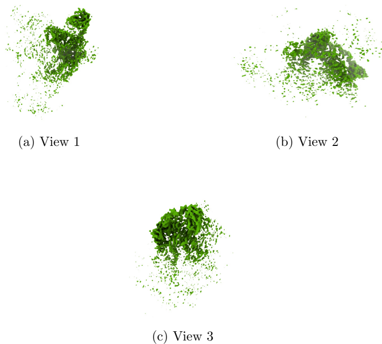
Figure 4: Isosurface at threshold=0.496800. Views generated by ChimeraX at a the following X, Y, Z angles: View 1 (0, -90, -90), View 2 (-90, 0, -90), View 3 (0, 0, 0).
