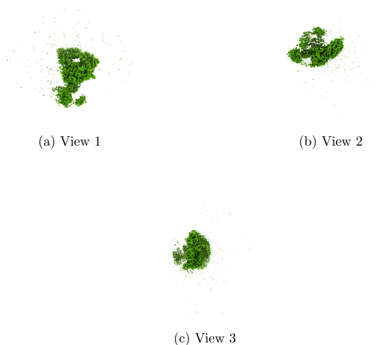
Figure 4: Isosurface at threshold=0.308000. Views generated by ChimeraX at a the following X, Y, Z angles: View 1 (0, -90, -90), View 2 (-90, 0, -90), View 3 (0, 0, 0).
