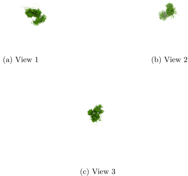
Figure 4: Isosurface at threshold=0.869100. Views generated by ChimeraX at a the following X, Y, Z angles: View 1 (0, -90, -90), View 2 (-90, 0, -90), View 3 (0, 0, 0).
