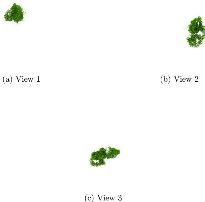
Figure 4: Isosurface at threshold=1.029000. Views generated by ChimeraX at a the following X, Y, Z angles: View 1 (0, -90, -90), View 2 (-90, 0, -90), View 3 (0, 0, 0).
