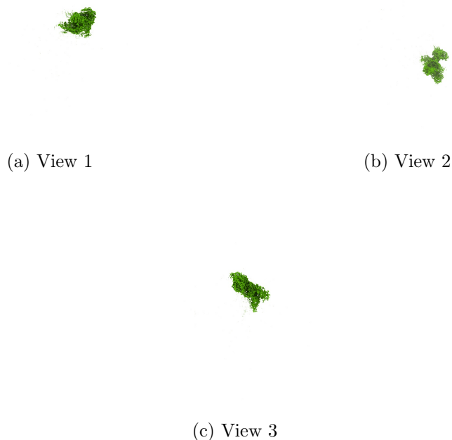
Figure 4: Isosurface at threshold=0.710000. Views generated by ChimeraX at a the following X, Y, Z angles: View 1 (0, -90, -90), View 2 (-90, 0, -90), View 3 (0, 0, 0).
