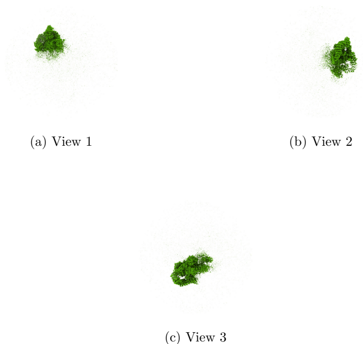
Figure 4: Isosurface at threshold=0.606000. Views generated by ChimeraX at a the following X, Y, Z angles: View 1 (0, -90, -90), View 2 (-90, 0, -90), View 3 (0, 0, 0).
