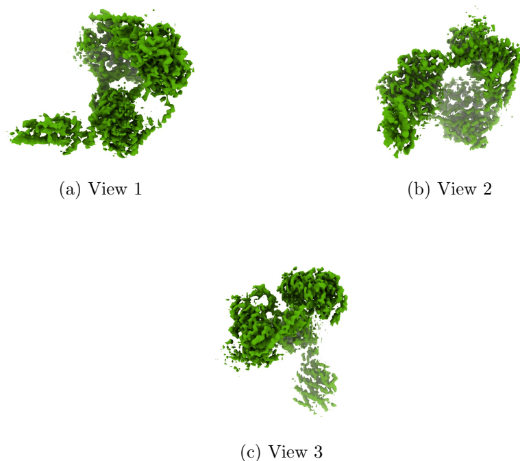
Figure 4: Isosurface at threshold=0.536500. Views generated by ChimeraX at a the following X, Y, Z angles: View 1 (0, -90, -90), View 2 (-90, 0, -90), View 3 (0, 0, 0).
