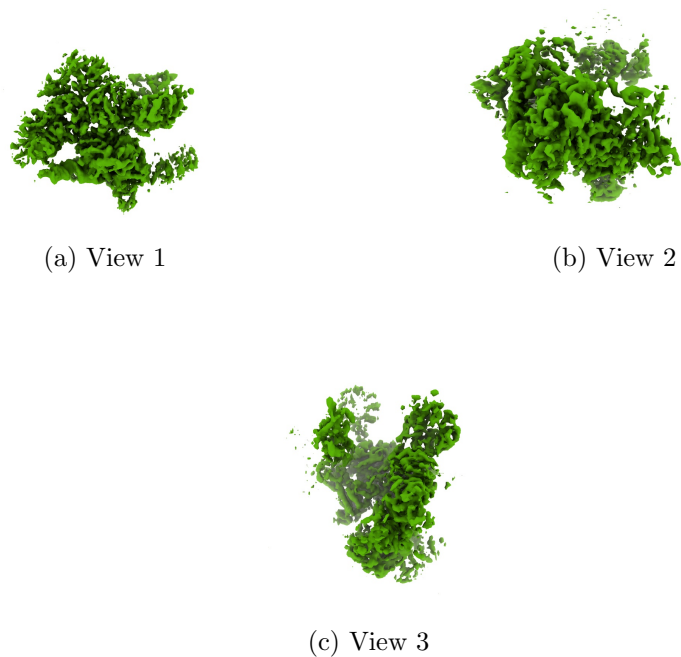
Figure 4: Isosurface at threshold=0.348900. Views generated by ChimeraX at a the following X, Y, Z angles: View 1 (0, -90, -90), View 2 (-90, 0, -90), View 3 (0, 0, 0).
