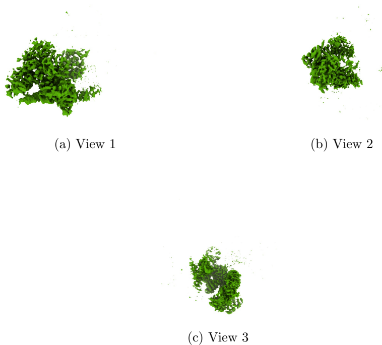
Figure 4: Isosurface at threshold=0.387500. Views generated by ChimeraX at a the following X, Y, Z angles: View 1 (0, -90, -90), View 2 (-90, 0, -90), View 3 (0, 0, 0).
