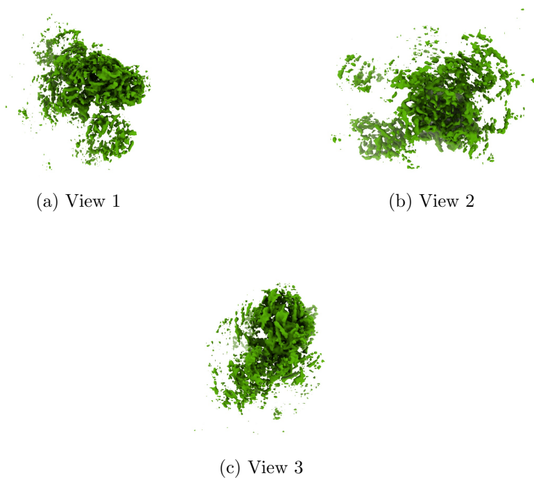
Figure 4: Isosurface at threshold=0.472400. Views generated by ChimeraX at a the following X, Y, Z angles: View 1 (0, -90, -90), View 2 (-90, 0, -90), View 3 (0, 0, 0).
