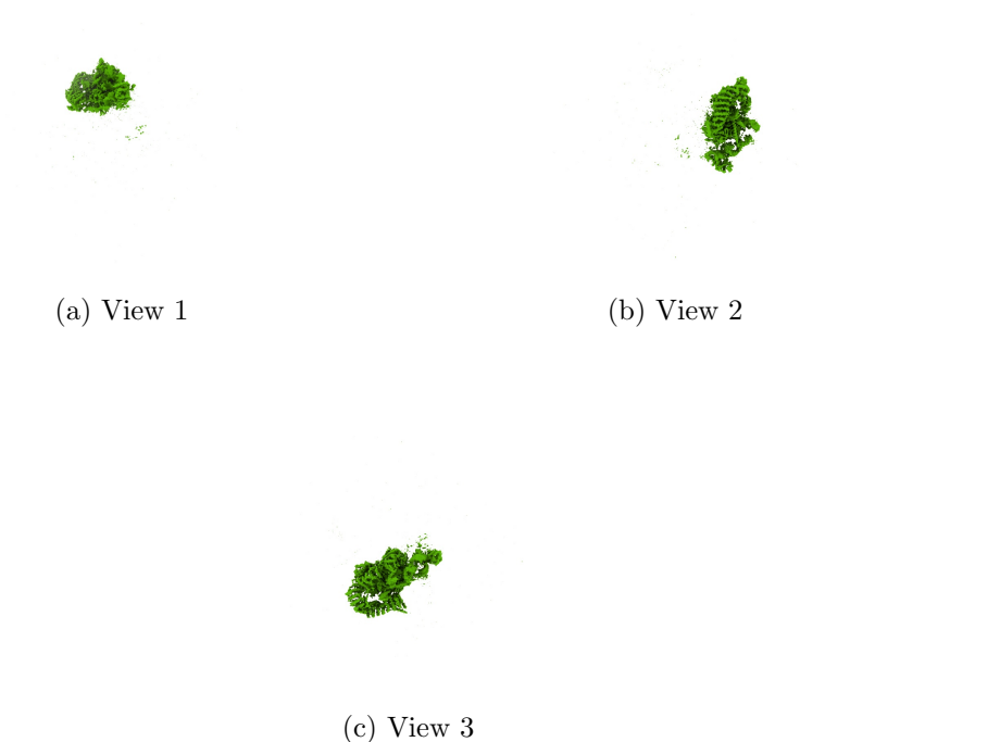
Figure 4: Isosurface at threshold=0.435900. Views generated by ChimeraX at a the following X, Y, Z angles: View 1 (0, -90, -90), View 2 (-90, 0, -90), View 3 (0, 0, 0).
