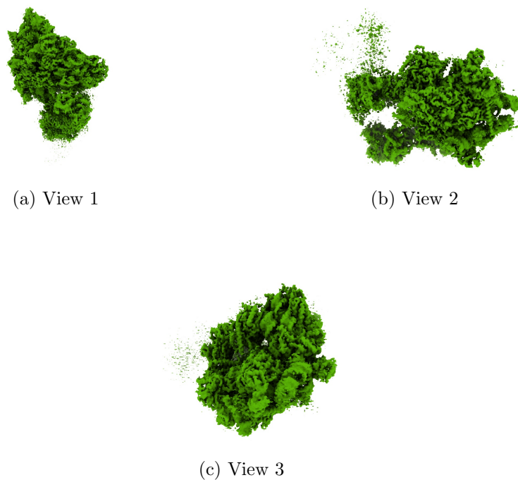
Figure 4: Isosurface at threshold=0.058010. Views generated by ChimeraX at a the following X, Y, Z angles: View 1 (0, -90, -90), View 2 (-90, 0, -90), View 3 (0, 0, 0).
