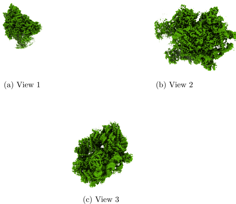
Figure 4: Isosurface at threshold=0.071510. Views generated by ChimeraX at a the following X, Y, Z angles: View 1 (0, -90, -90), View 2 (-90, 0, -90), View 3 (0, 0, 0).
