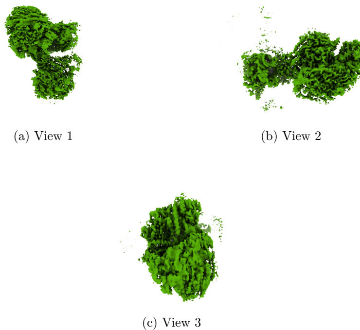
Figure 4: Isosurface at threshold=0.062400. Views generated by ChimeraX at a the following X, Y, Z angles: View 1 (0, -90, -90), View 2 (-90, 0, -90), View 3 (0, 0, 0).
