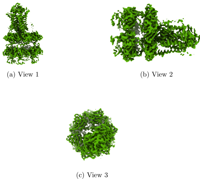
Figure 4: Isosurface at threshold=0.009250. Views generated by ChimeraX at a the following X, Y, Z angles: View 1 (0, -90, -90), View 2 (-90, 0, -90), View 3 (0, 0, 0).
