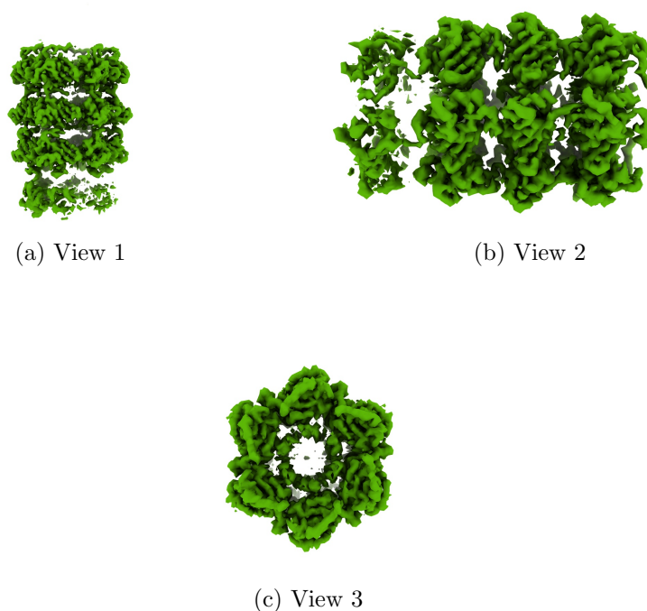
Figure 4: Isosurface at threshold=0.137000. Views generated by ChimeraX at a the following X, Y, Z angles: View 1 (0, -90, -90), View 2 (-90, 0, -90), View 3 (0, 0, 0).
