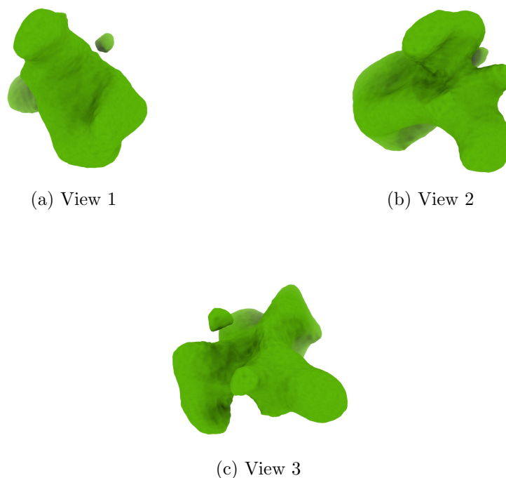
Figure 4: Isosurface at threshold=0.016100. Views generated by ChimeraX at a the following X, Y, Z angles: View 1 (0, -90, -90), View 2 (-90, 0, -90), View 3 (0, 0, 0).
