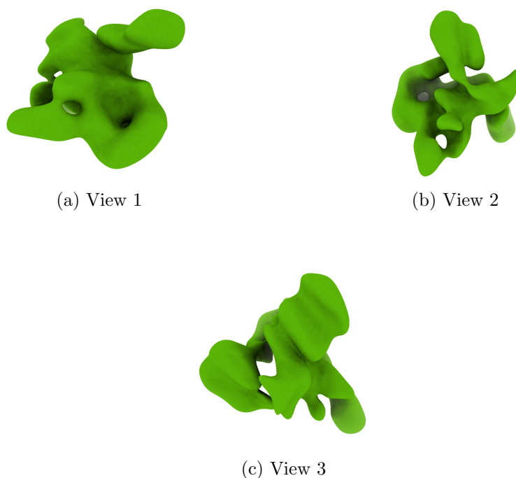
Figure 4: Isosurface at threshold=0.017200. Views generated by ChimeraX at a the following X, Y, Z angles: View 1 (0, -90, -90), View 2 (-90, 0, -90), View 3 (0, 0, 0).
