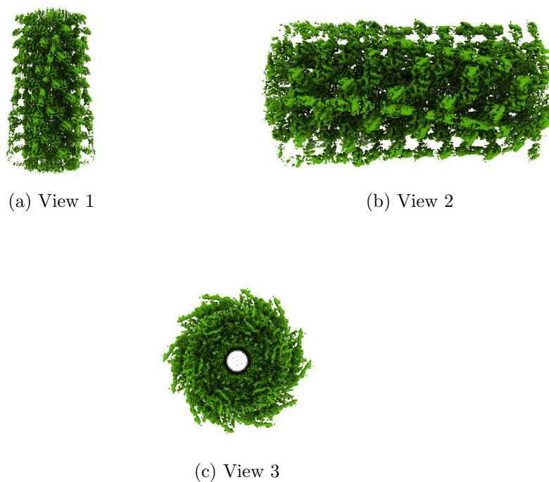
Figure 4: Isosurface at threshold=0.903000. Views generated by ChimeraX at a the following X, Y, Z angles: View 1 (0, -90, -90), View 2 (-90, 0, -90), View 3 (0, 0, 0).
