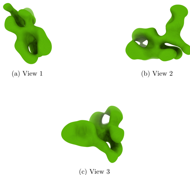
Figure 4: Isosurface at threshold=0.025300. Views generated by ChimeraX at a the following X, Y, Z angles: View 1 (0, -90, -90), View 2 (-90, 0, -90), View 3 (0, 0, 0).
