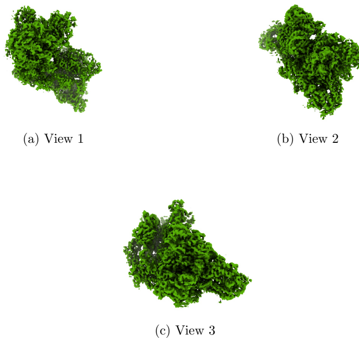
Figure 4: Isosurface at threshold=0.015100. Views generated by ChimeraX at a the following X, Y, Z angles: View 1 (0, -90, -90), View 2 (-90, 0, -90), View 3 (0, 0, 0).
