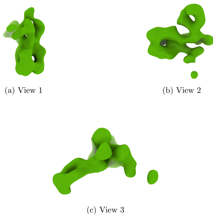
Figure 4: Isosurface at threshold=0.018700. Views generated by ChimeraX at a the following X, Y, Z angles: View 1 (0, -90, -90), View 2 (-90, 0, -90), View 3 (0, 0, 0).
