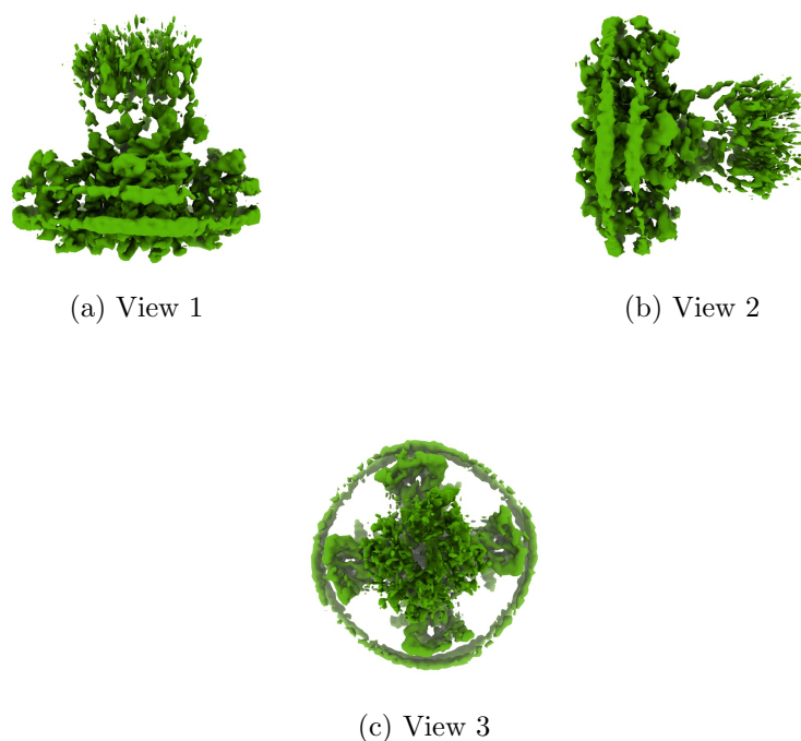
Figure 4: Isosurface at threshold=0.219000. Views generated by ChimeraX at a the following X, Y, Z angles: View 1 (0, -90, -90), View 2 (-90, 0, -90), View 3 (0, 0, 0).
