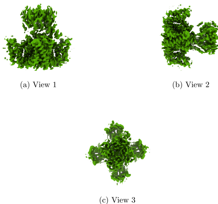
Figure 4: Isosurface at threshold=0.126000. Views generated by ChimeraX at a the following X, Y, Z angles: View 1 (0, -90, -90), View 2 (-90, 0, -90), View 3 (0, 0, 0).
