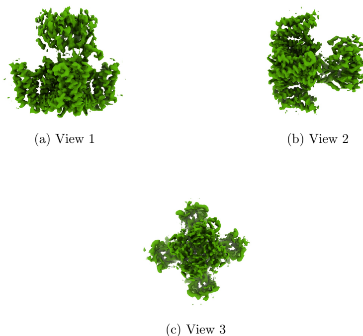
Figure 4: Isosurface at threshold=0.121000. Views generated by ChimeraX at a the following X, Y, Z angles: View 1 (0, -90, -90), View 2 (-90, 0, -90), View 3 (0, 0, 0).
