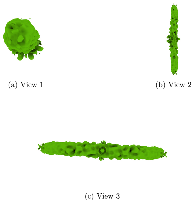
Figure 4: Isosurface at threshold=0.032700. Views generated by ChimeraX at a the following X, Y, Z angles: View 1 (0, -90, -90), View 2 (-90, 0, -90), View 3 (0, 0, 0).
