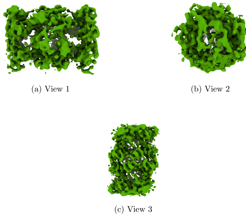
Figure 4: Isosurface at threshold=0.269000. Views generated by ChimeraX at a the following X, Y, Z angles: View 1 (0, -90, -90), View 2 (-90, 0, -90), View 3 (0, 0, 0).
