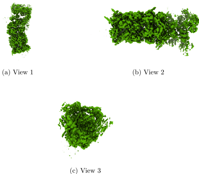
Figure 4: Isosurface at threshold=0.176000. Views generated by ChimeraX at a the following X, Y, Z angles: View 1 (0, -90, -90), View 2 (-90, 0, -90), View 3 (0, 0, 0).
