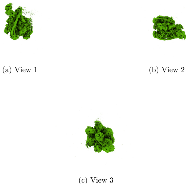
Figure 4: Isosurface at threshold=0.007500. Views generated by ChimeraX at a the following X, Y, Z angles: View 1 (0, -90, -90), View 2 (-90, 0, -90), View 3 (0, 0, 0).
