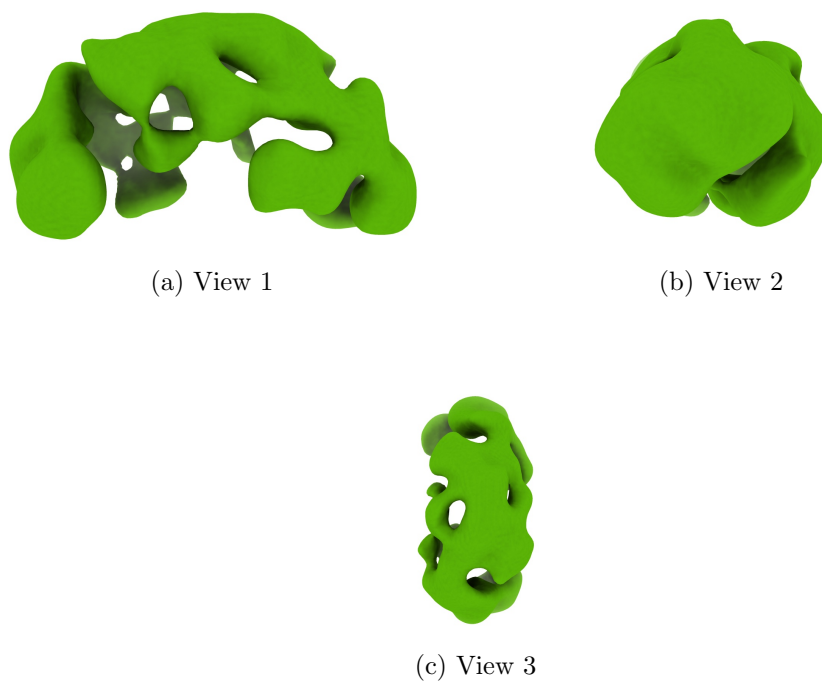
Figure 4: Isosurface at threshold=0.028500. Views generated by ChimeraX at a the following X, Y, Z angles: View 1 (0, -90, -90), View 2 (-90, 0, -90), View 3 (0, 0, 0).
