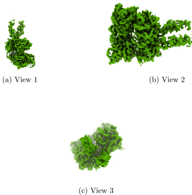
Figure 4: Isosurface at threshold=0.470000. Views generated by ChimeraX at a the following X, Y, Z angles: View 1 (0, -90, -90), View 2 (-90, 0, -90), View 3 (0, 0, 0).
