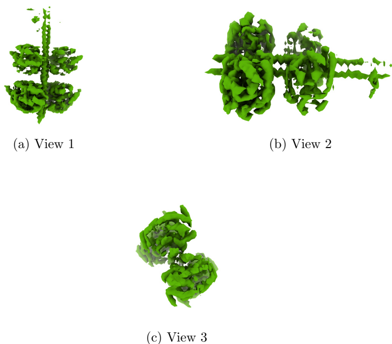
Figure 4: Isosurface at threshold=0.209000. Views generated by ChimeraX at a the following X, Y, Z angles: View 1 (0, -90, -90), View 2 (-90, 0, -90), View 3 (0, 0, 0).
