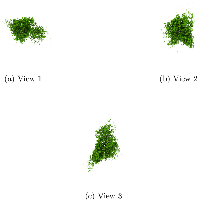
Figure 4: Isosurface at threshold=0.114000. Views generated by ChimeraX at a the following X, Y, Z angles: View 1 (0, -90, -90), View 2 (-90, 0, -90), View 3 (0, 0, 0).
