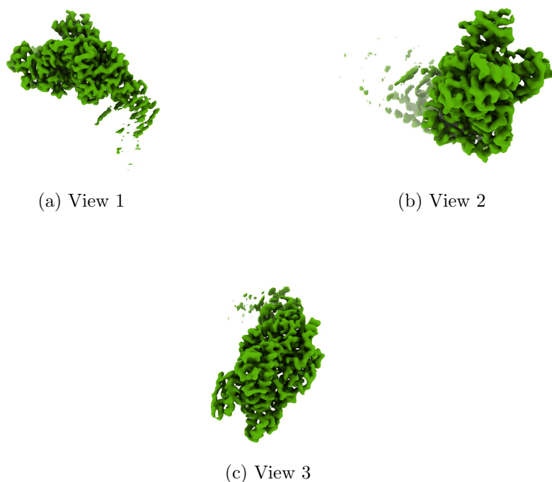
Figure 4: Isosurface at threshold=0.037200. Views generated by ChimeraX at a the following X, Y, Z angles: View 1 (0, -90, -90), View 2 (-90, 0, -90), View 3 (0, 0, 0).
