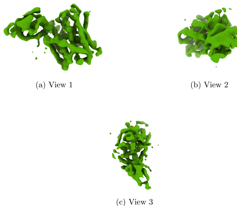
Figure 4: Isosurface at threshold=0.640000. Views generated by ChimeraX at a the following X, Y, Z angles: View 1 (0, -90, -90), View 2 (-90, 0, -90), View 3 (0, 0, 0).
