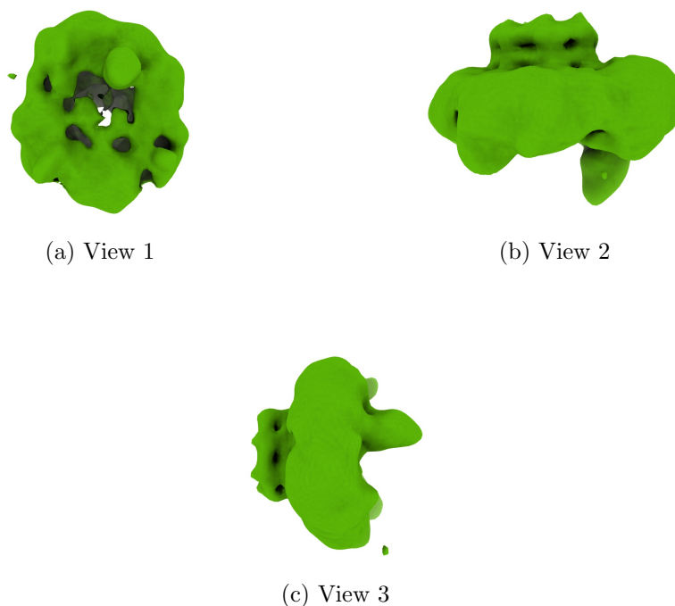
Figure 4: Isosurface at threshold=1.360000. Views generated by ChimeraX at a the following X, Y, Z angles: View 1 (0, -90, -90), View 2 (-90, 0, -90), View 3 (0, 0, 0).
