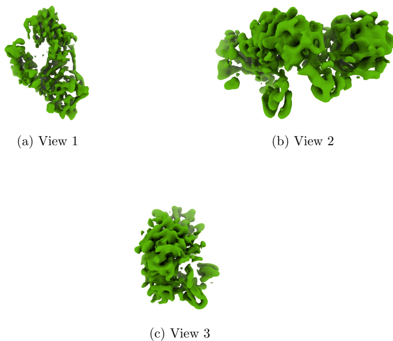
Figure 4: Isosurface at threshold=0.251000. Views generated by ChimeraX at a the following X, Y, Z angles: View 1 (0, -90, -90), View 2 (-90, 0, -90), View 3 (0, 0, 0).
