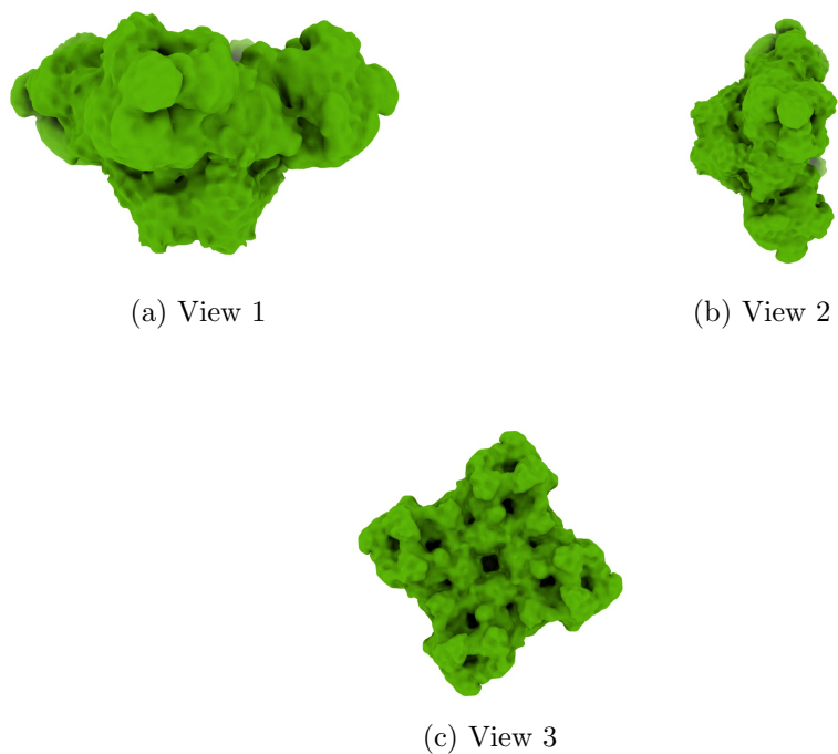
Figure 4: Isosurface at threshold=0.070700. Views generated by ChimeraX at a the following X, Y, Z angles: View 1 (0, -90, -90), View 2 (-90, 0, -90), View 3 (0, 0, 0).
