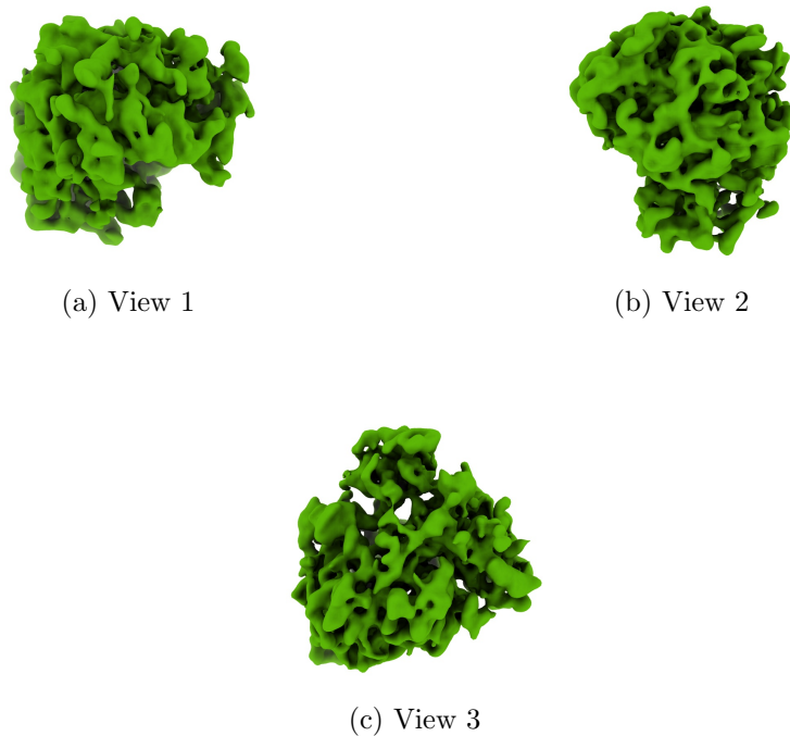
Figure 4: Isosurface at threshold=65.200000. Views generated by ChimeraX at a the following X, Y, Z angles: View 1 (0, -90, -90), View 2 (-90, 0, -90), View 3 (0, 0, 0).
